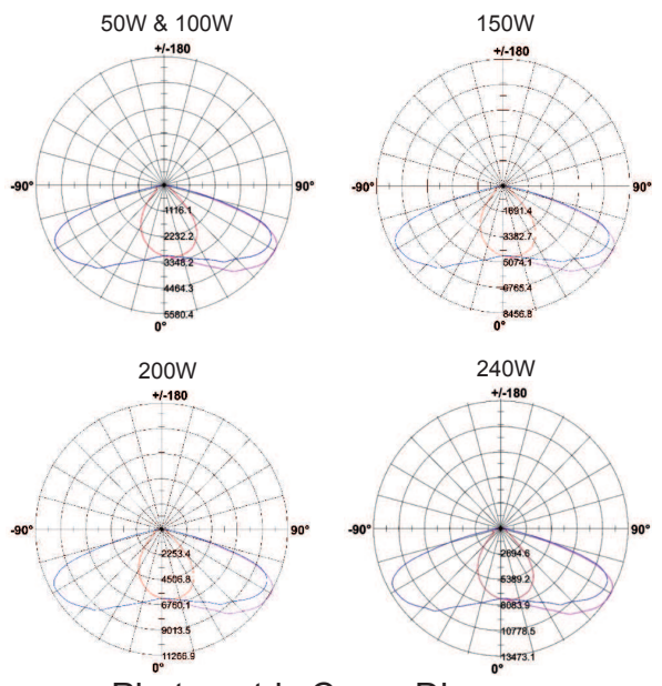
Photometric Curve Diagram
